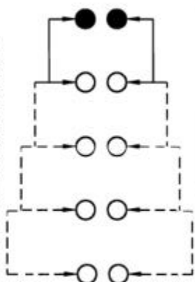
SCHEMATIC (NON-SHORTING)
